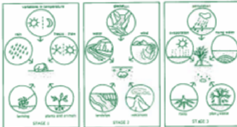
Three stages of decomposition of rock through interaction of different influences.
