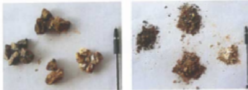
These pictures show four different types of rock, which were found in the samples of Pachhaiya. They could all be crumbled simply by hand.
